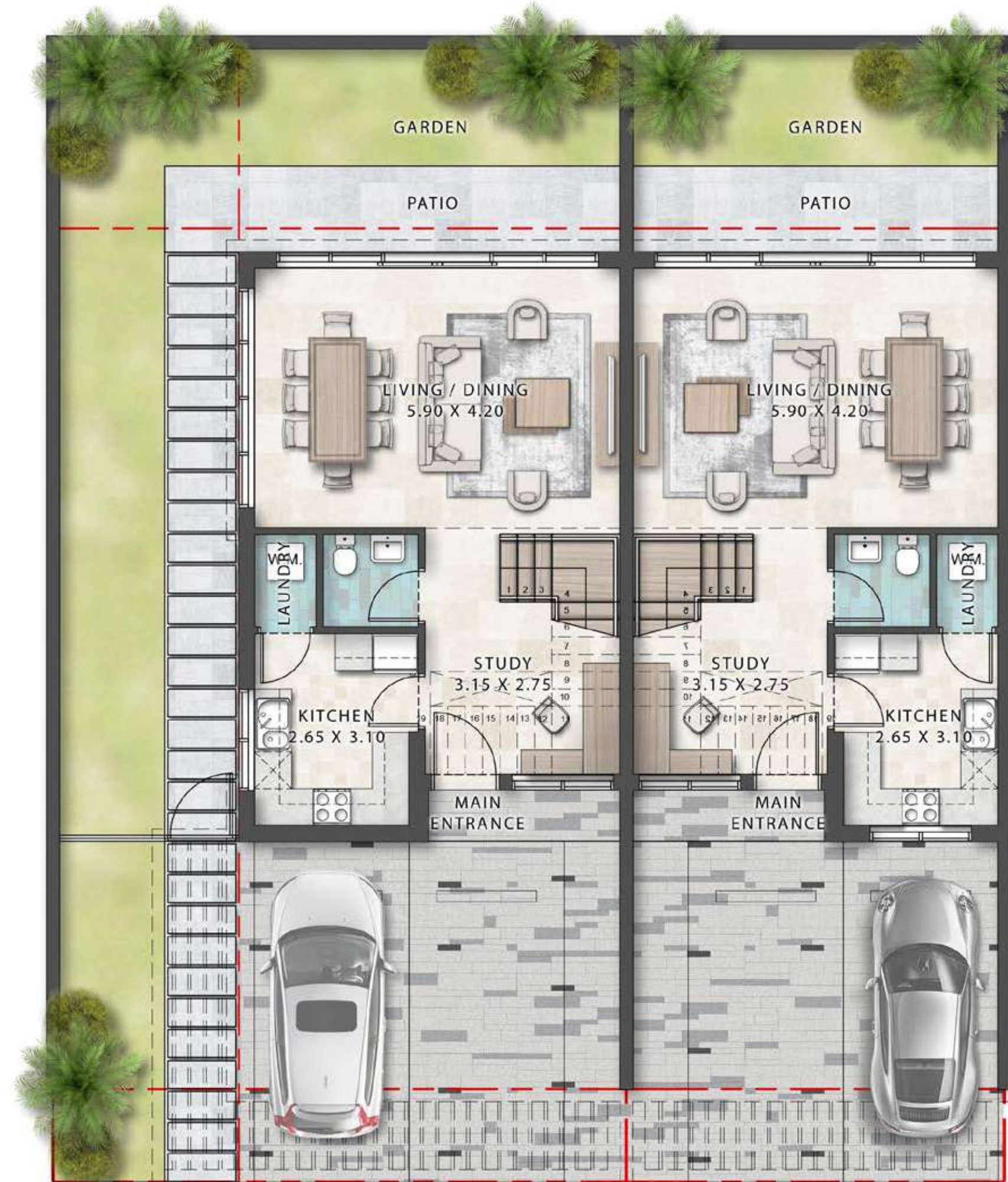
GROUND FLOOR
